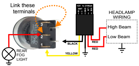
Wiring for: SAVAGE / APEM Aluminium Rear Fog Light Switch
